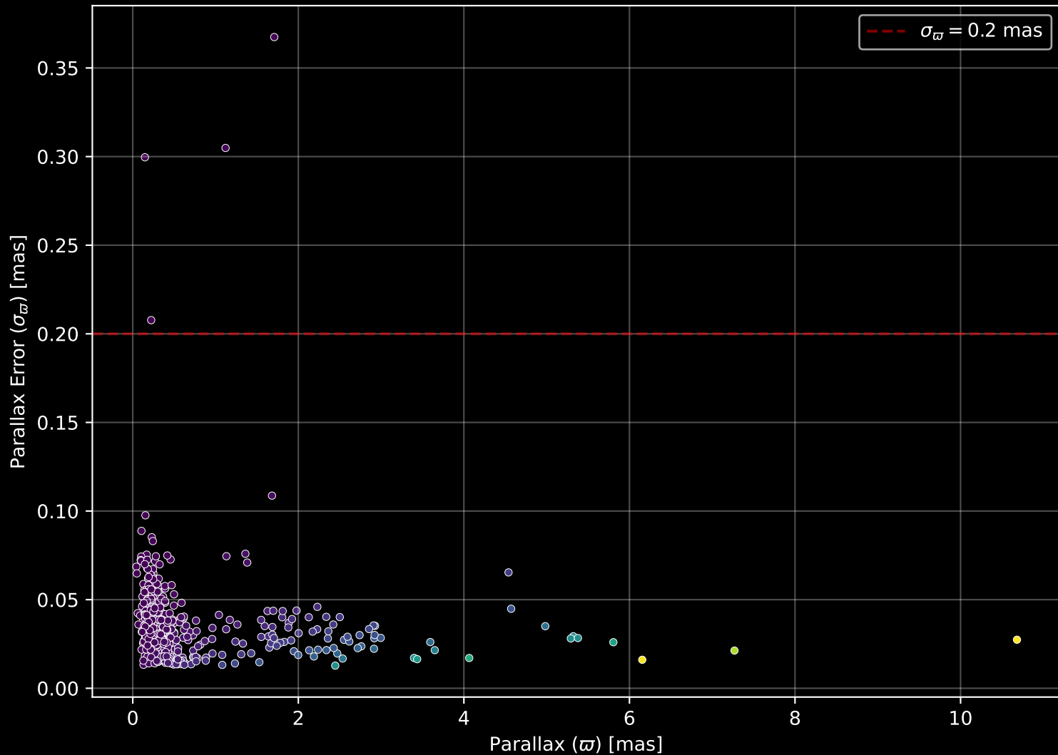
APOGEE DR17 Field: [150-04] Parallax Quality (n= 483)
