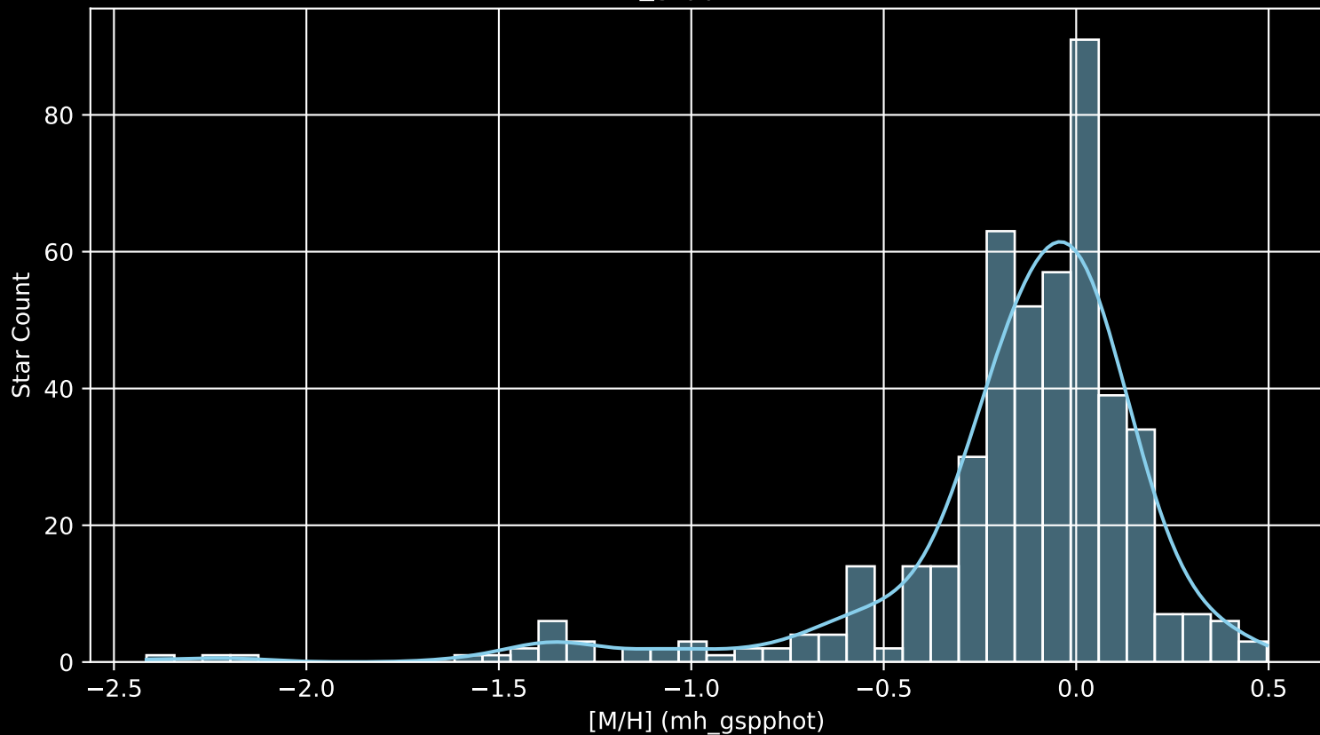
APOGEE DR17 Field: [150-04 [M/H] (mh_gspphot) (n= 469)
