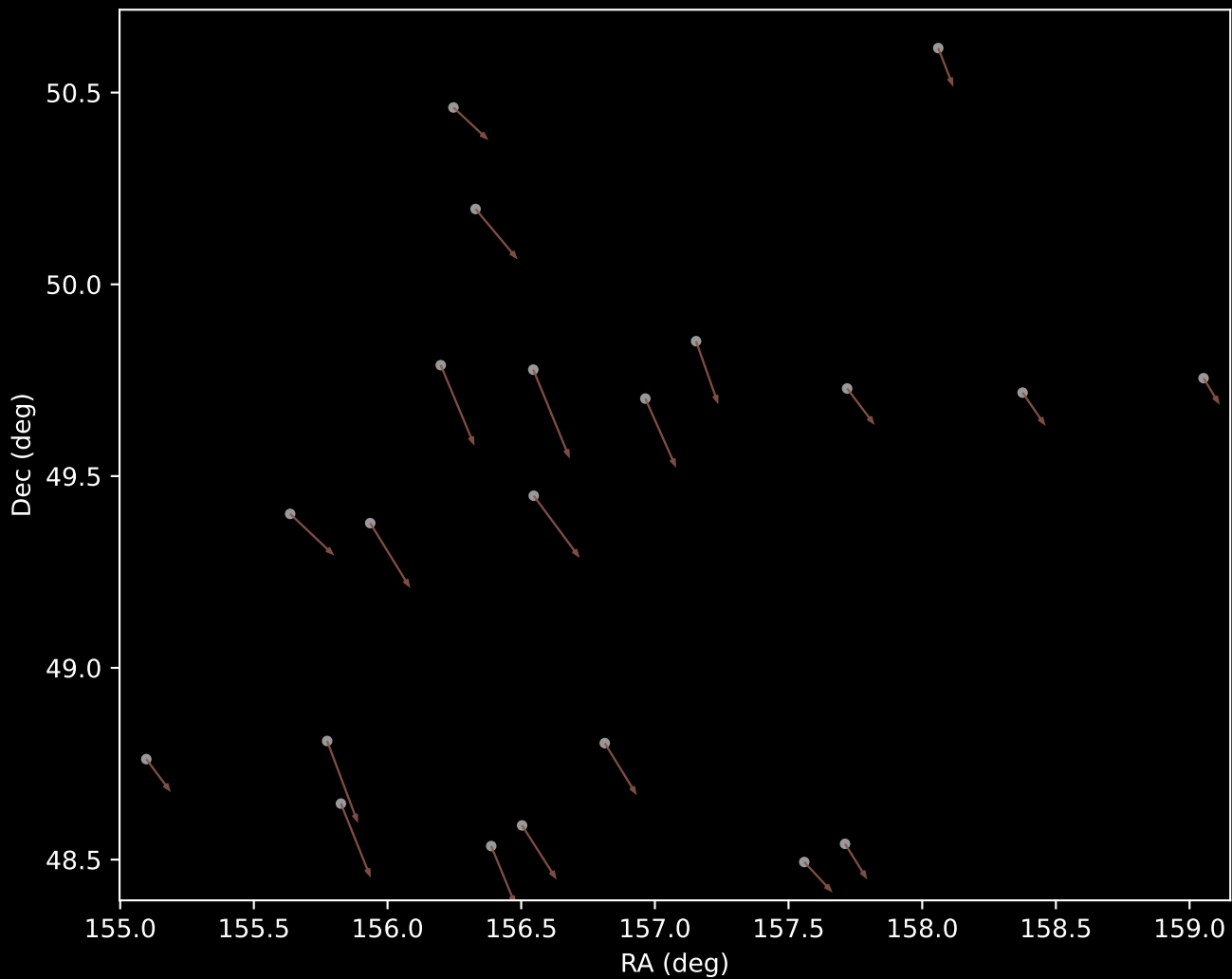
APOGEE DR17 Cluster 10 Proper Motion Vectors (n=21)
