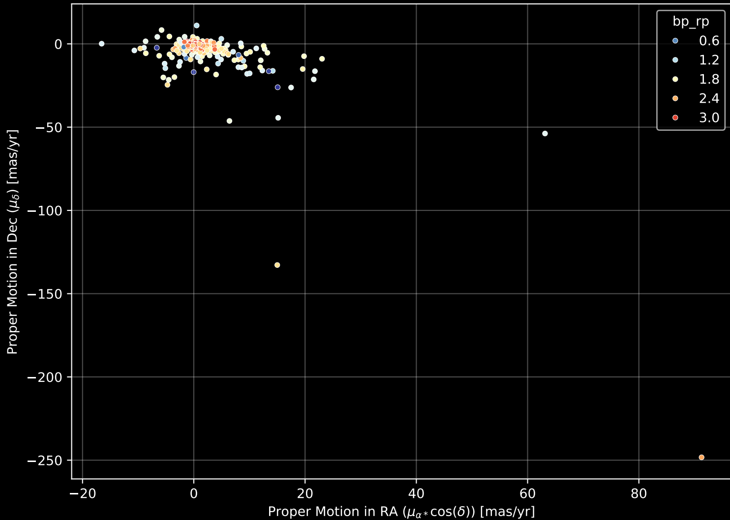
APOGEE DR17 Field: [150-04] Proper Motion Diagram (n= 483)
