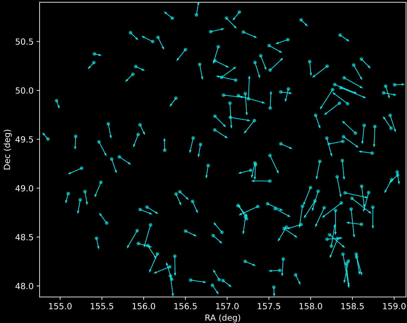
APOGEE DR17 Noise Stream Proper Motion Vectors (n=152)
