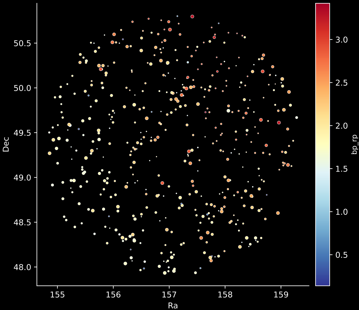
APOGEE DR17 Field: [150-04] Stars: 483
