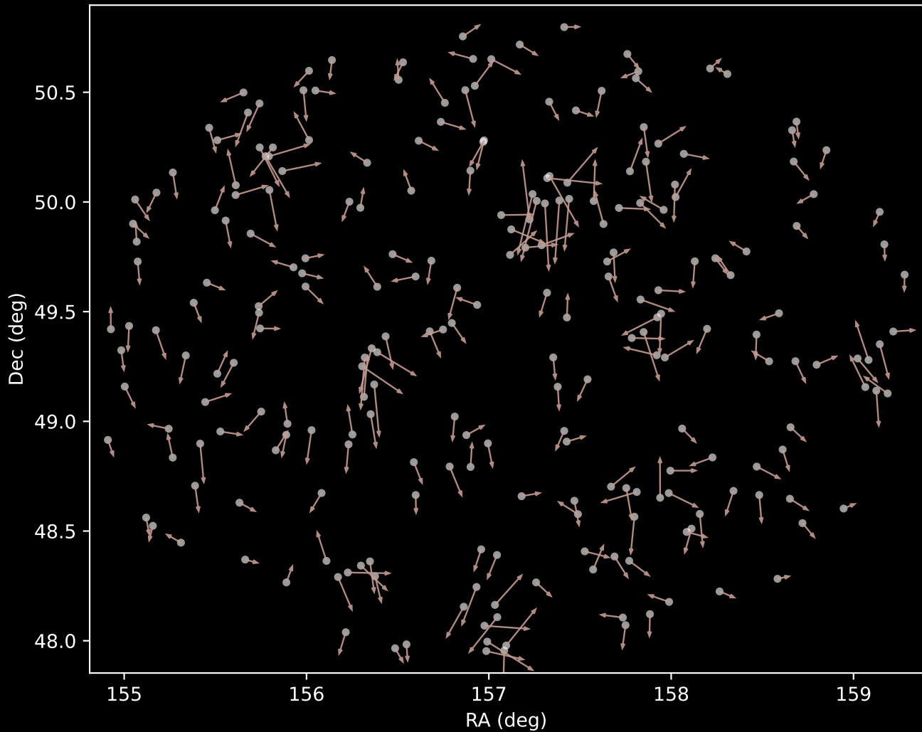
APOGEE DR17 Cluster 11 Proper Motion Vectors (n=240)
