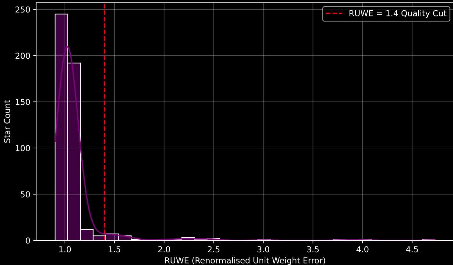
GAPOGEE DR17 Field [150-04] RUWE Distribution (n= 479)
